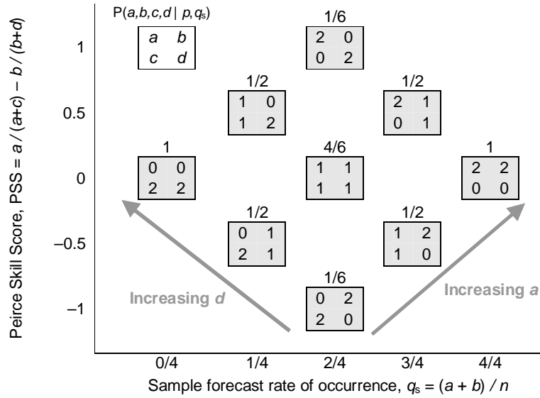
Figure 1. The possible contingency tables for number of forecasts n = 4 and base rate p = 1/2 , as a function of the sample forecast rate of occurrence q_s and the Peirce Skill Score. The elements of the contingency tables are a-d as shown in the white table to the top left. The numbers above each box give P(a, b, c, d | p, q_s) , the probability of that table occurring randomly given one has a particular base rate and sample forecast rate of occurrence q_s . Therefore these conditional probabilities sum to one in each column.
