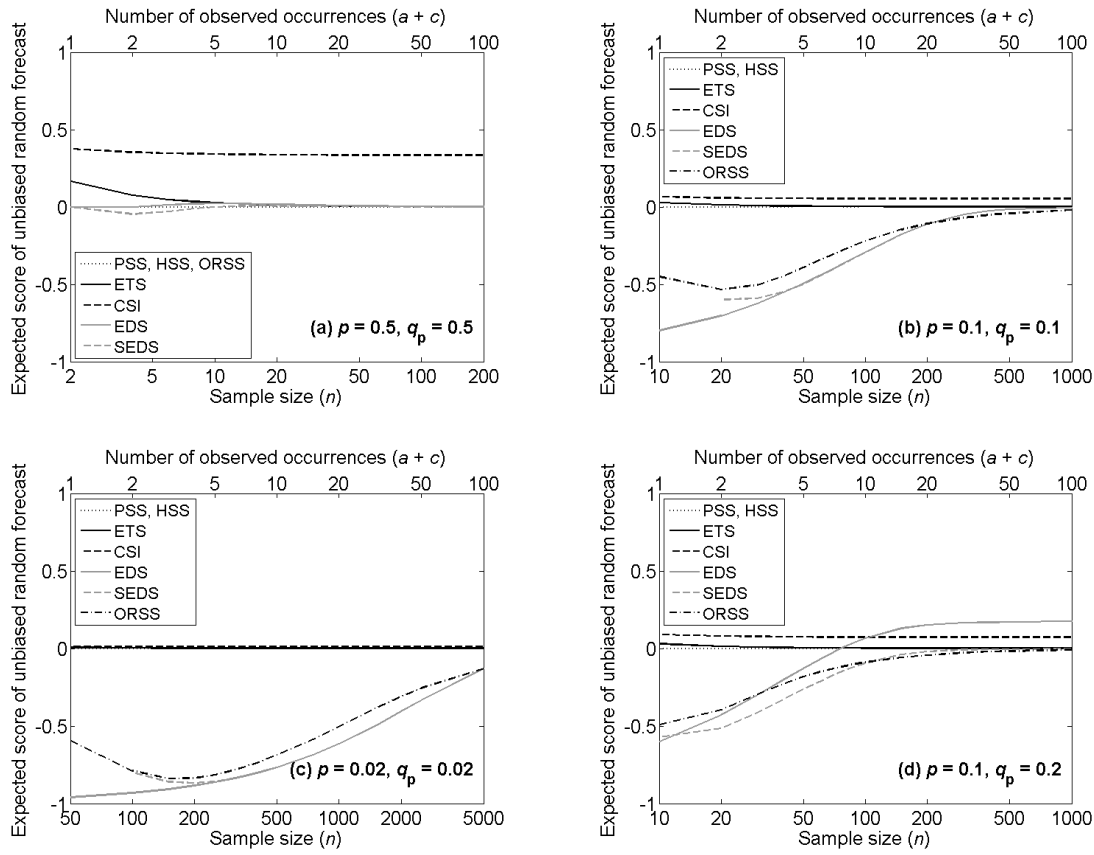
Figure 5. The expected values of a number of verification measures, E(S|p) , versus sample size, for random forecasting systems with base rate p and population forecast probability of occurrence q_p of (a) p = q_p = 0.5 , (b) p = q_p = 0.1 , (c) p = q_p = 0.02 , and (d) p = 0.1 and q_p = 0.2 . The undefined values are removed from consideration when calculating SEDS, but when these occupy more than 25% of probability space, SEDS is not plotted; this only affects panels b and d.
