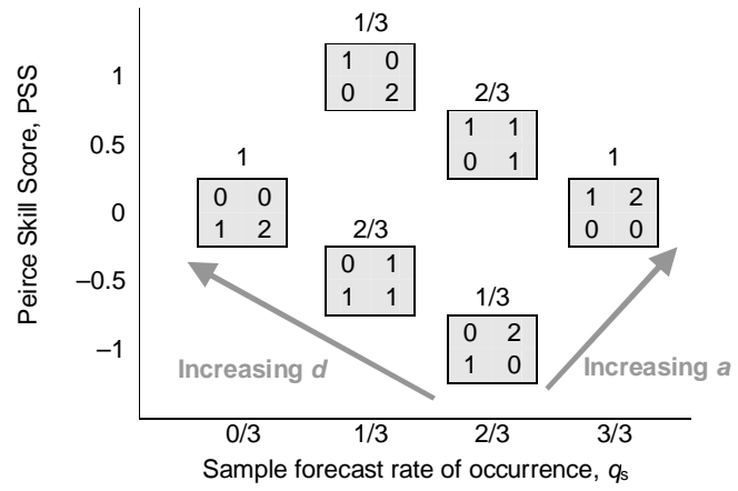
Figure 3. As Fig. 1 but for number of forecasts n = 3 and base rate p = 1/3 .
