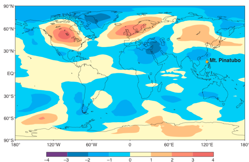
Lower tropospheric temperature anomalies during winter 1991/2 following Mt Pinatubo eruption during summer 1991. Taken from Robock, Science (2002).
