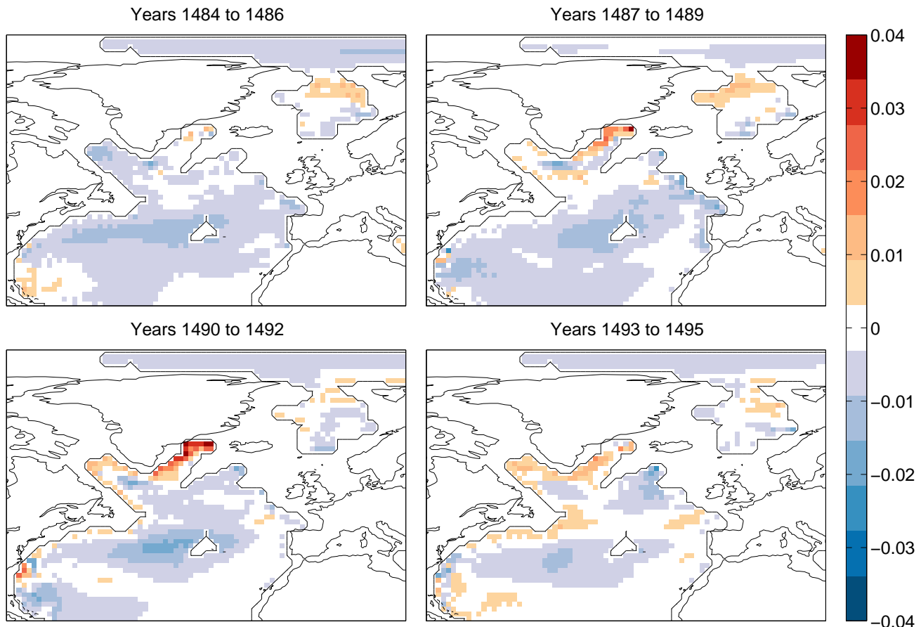
Figure 4. Integrated density anomalies from 800m to 3000m, relative to the control run mean, for averaged 3 year periods as labelled. The thin black contour is the 3000m isobath in HadCM3. Note the different years to Fig. 3.
