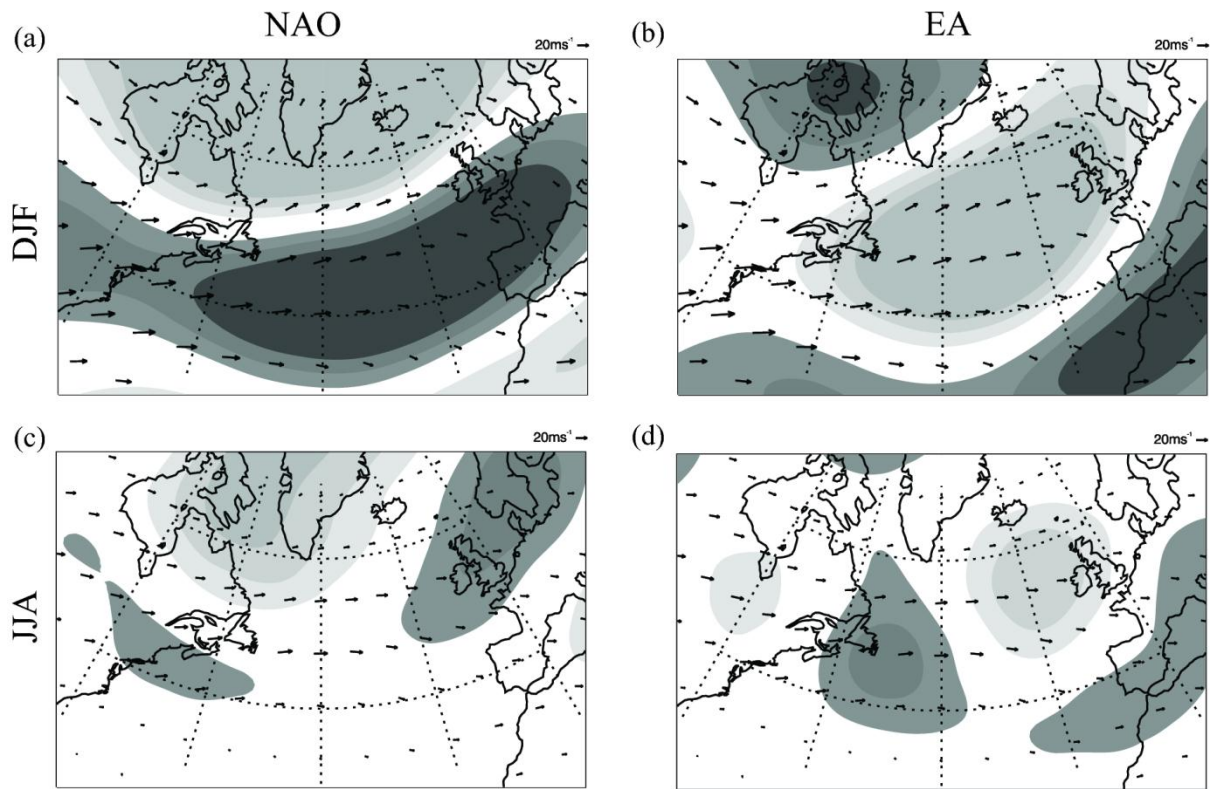
Figure 5: Northern hemisphere teleconnection patterns defined from ERA-Interim data for (a) and (b) winter and (c) and (d) summer. The North Atlantic Oscillation, NAO, pattern ((a), (c)) and East Atlantic, EA, pattern ((b), (d)) are shown in their positive phases. The contours represent positive (dark grey) and negative (light grey) geopotential height or pressure anomalies at 250 hPa. The climatological wind vectors are also plotted in each panel.
