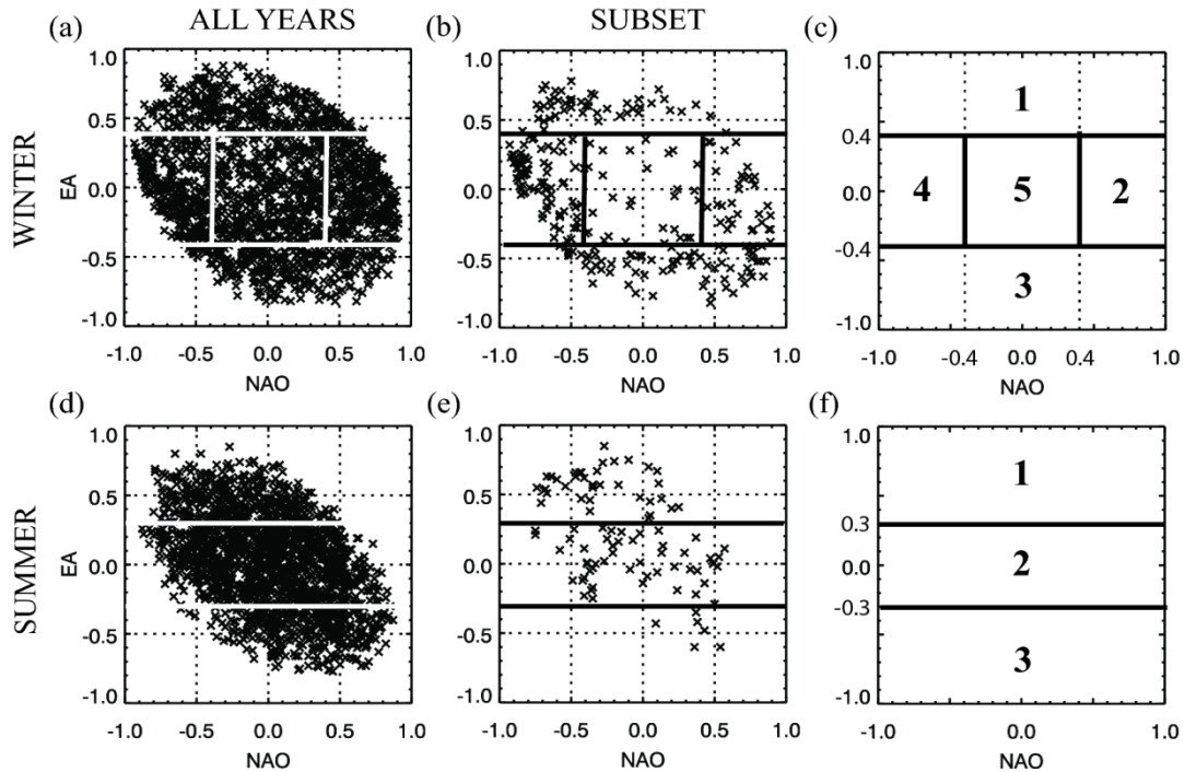
Figure 6: Scatterplot of the projection coefficients obtained by projecting daily Z250 anomalies of ERA-Interim data onto the NAO and EA patterns in winter ((a)-(b)) and summer ((d)-(e)). (a) and (d) show the projection coefficients for all years in ERA-Interim; (b) and (e) show the years for which optimum route data is available for that season (i.e., 2004-05, 2008-09 and 2009-10 for (b) and 2009 for (e)). (c) and (f) show the thresholds used to split the data into 5 types in winter and 3 in summer.
