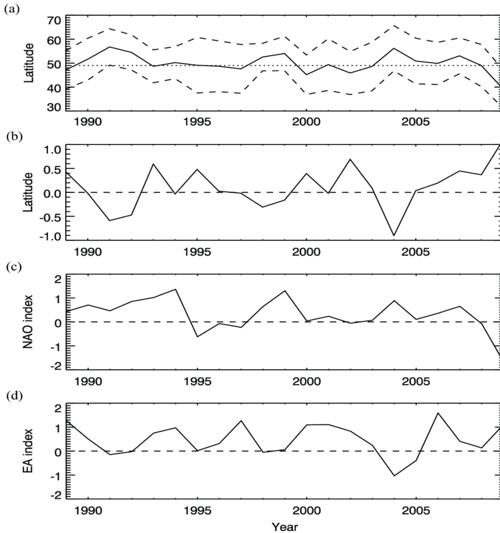
Figure 1: (a) Time series of the winter (DJF) mean jet latitude in ERA-Interim (solid line) and the intra-seasonal standard deviation (dashed lines). The 1989-2009 winter mean jet latitude is overlaid on (a) (dotted line). (b) The time-series of the intra-seasonal skewness of the winter jet latitude in ERA-Interim. Time series of (c) NAO index and (d) EA index for the same period. The year on the axes corresponds to the December of each winter.
