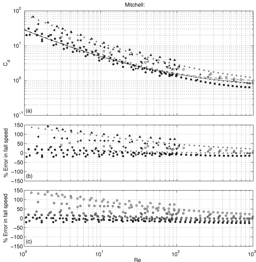
FIG. 2. Tank experiment data. (a) Comparison of experimental Re-X data (symbols) with theoretical curve of Mitchell (1996; solid line), Mitchell and Heymsfield (2005; dashed line), and Khvorostyanov and Curry (2005; dotted line). (b) Corresponding relative error in fall speed for a given Re if Mitchell's curve is assumed. (c) As in (b), but symbols are now replaced by circles filled with different shades of gray, with darker shades symbolizing larger A_r ( A_r = 1 is black and A_r = 0 is white). Symbols in (a) and (b) are as follows. Planar types are filled: disc is a circle, hexagonal plate is a diamond, broad-branch crystal is a right-pointing triangle, plate with extensions is a down-pointing triangle, dendrite is a left-pointing triangle, and stellar is an up-pointing triangle. Thick disc (aspect ratio 0.5) is a black pentagram. Cylinders with aspect ratio: 10 is a plus sign, 5 is an asterisk, 2 is an ex, and 1 is a black filled square. Aggregates are open: cross shape is a circle, H shape is a square, star shape is a hexagram, and chain is a pentagram. See text for more details.
