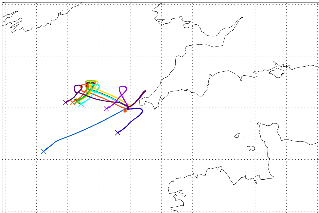
Balloon launch 12UT 02/09/2003 000hr met forecast
