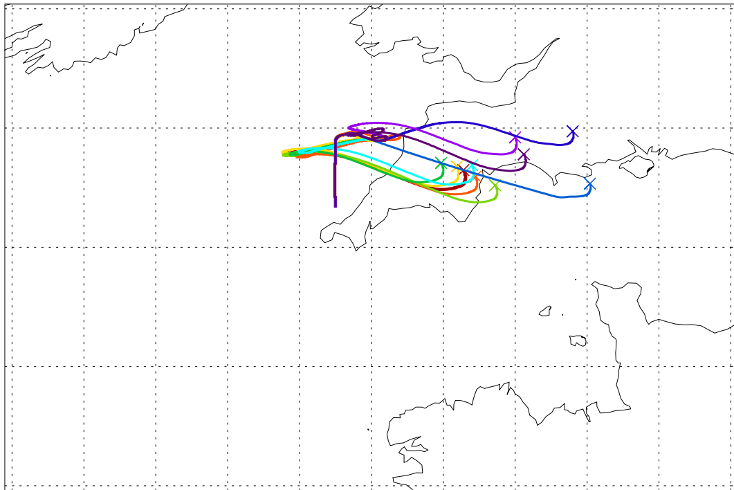
Balloon launch 12UT 07/09/2003 000hr met forecast
