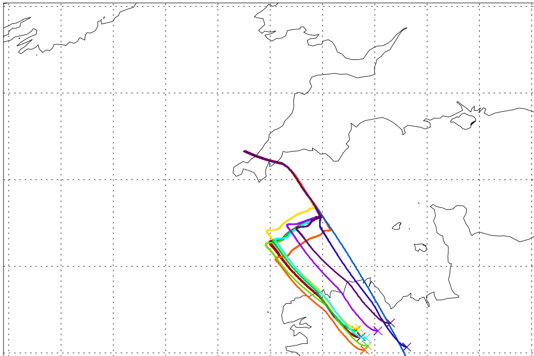
Balloon launch 12UT 09/09/2003 000hr met forecast
