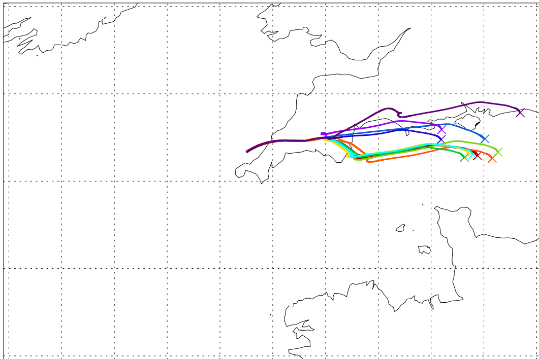
Balloon launch 12UT 11/09/2003 000hr met forecast
