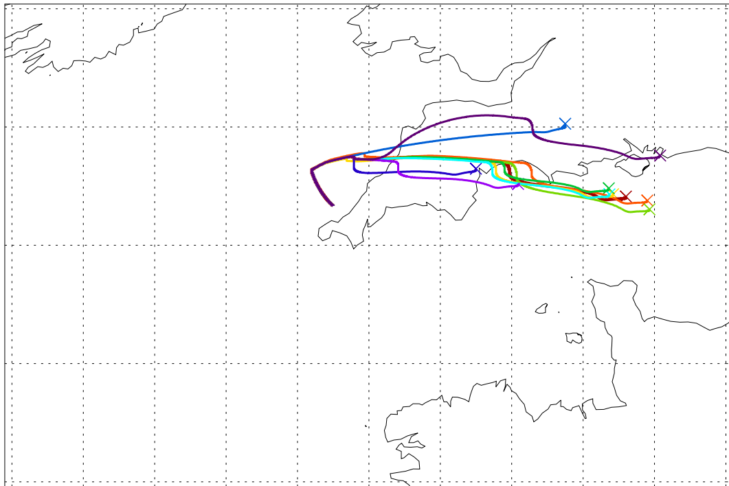
Balloon launch 12UT 15/09/2003 000hr met forecast
