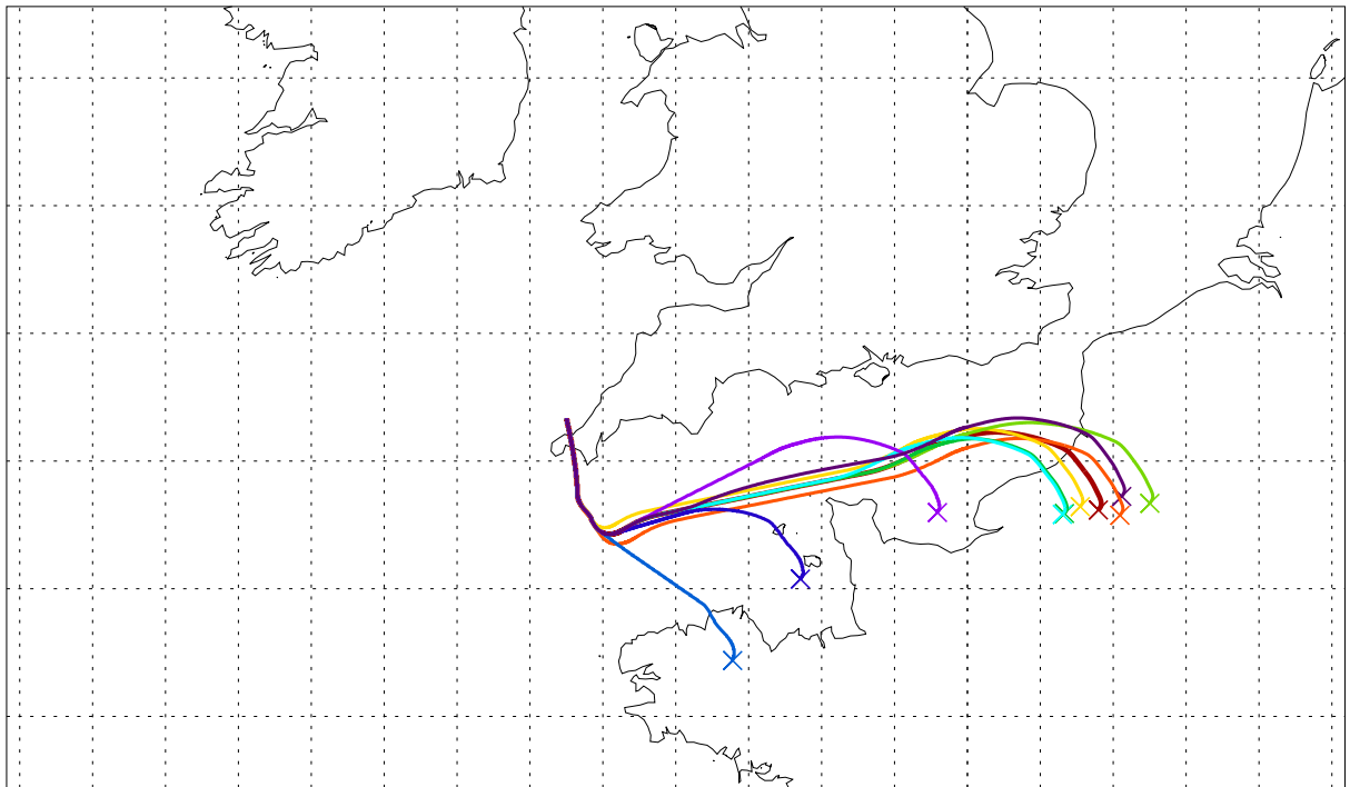
Balloon launch 12UT 23/09/2003 000hr met forecast
