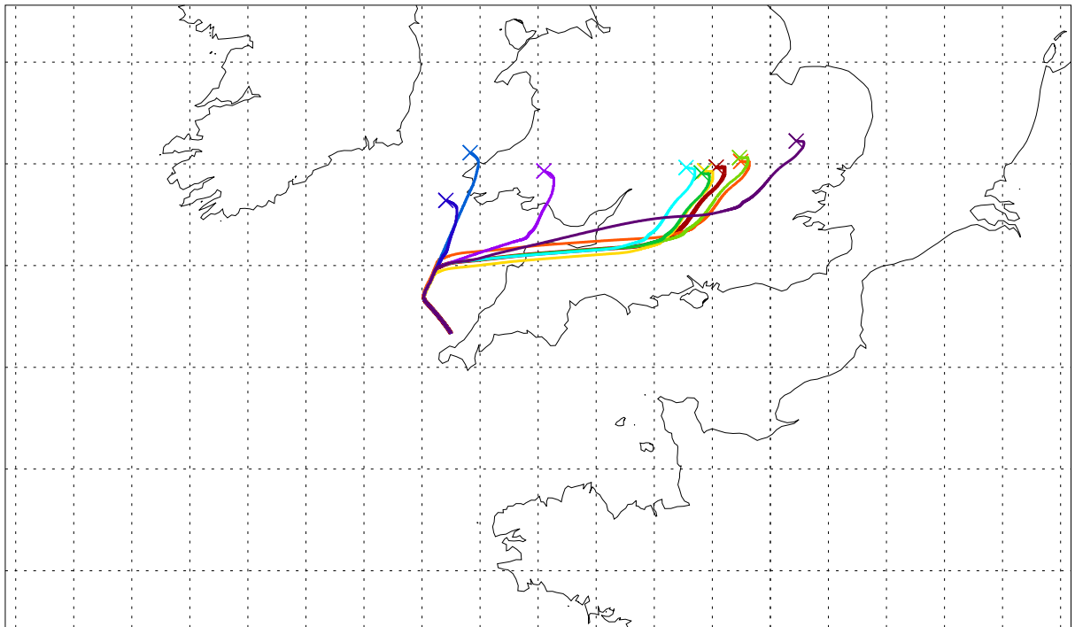
Balloon launch 12UT 30/09/2003 000hr met forecast
