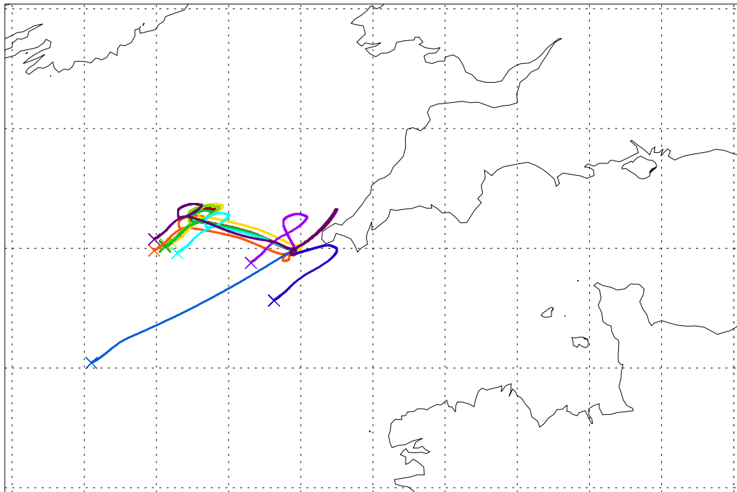
Balloon launch 12UT 02/09/2003 024hr met forecast
