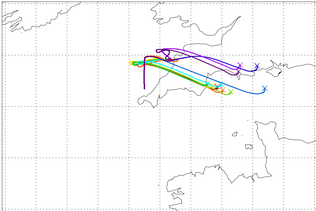
Balloon launch 12UT 07/09/2003 024hr met forecast
