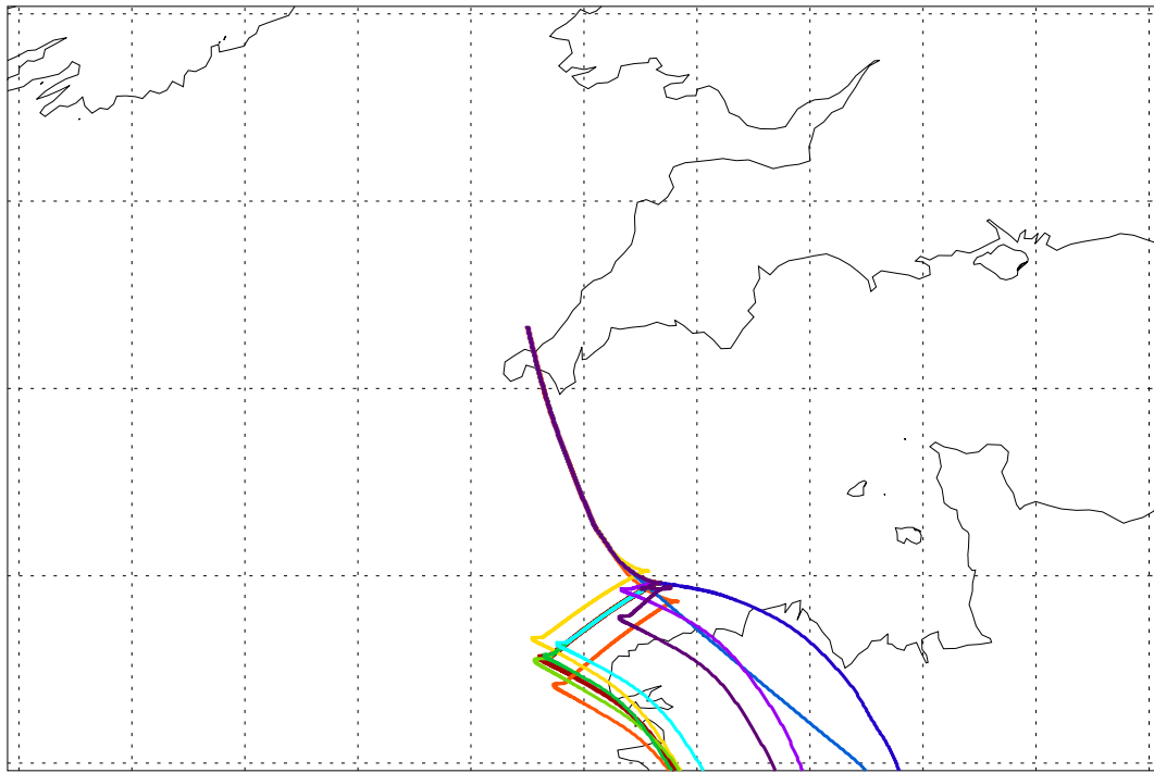
Balloon launch 12UT 08/09/2003 024hr met forecast
