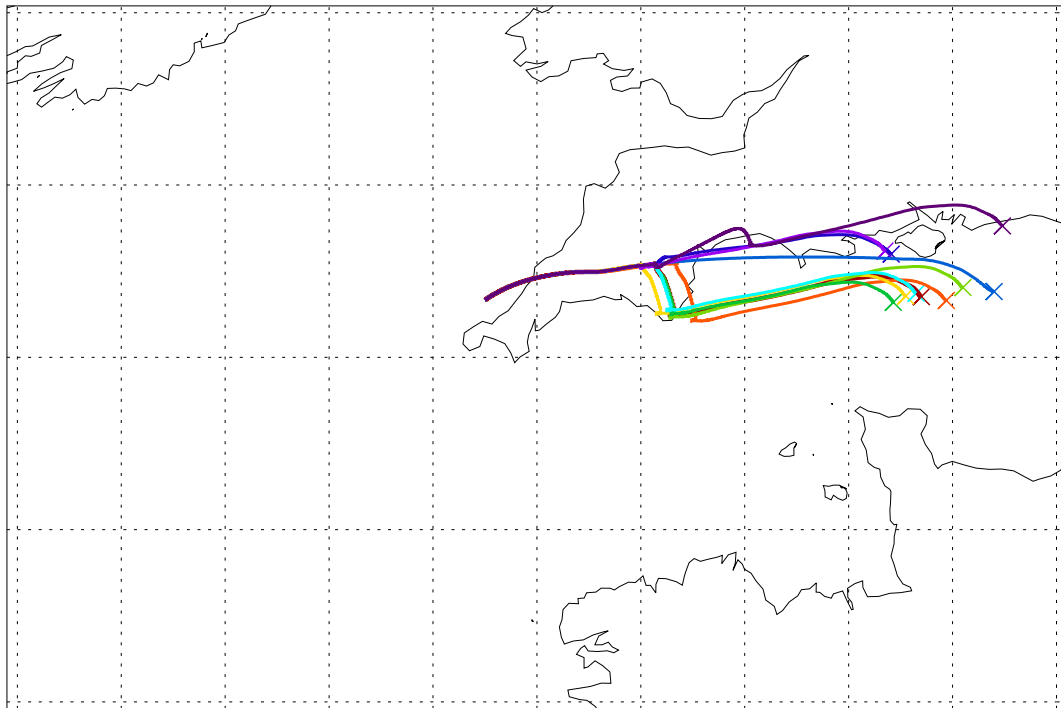
Balloon launch 12UT 11/09/2003 024hr met forecast
