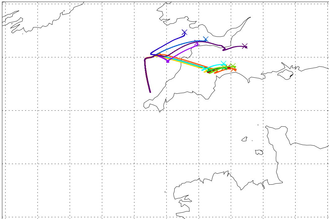
Balloon launch 12UT 13/09/2003 024hr met forecast
