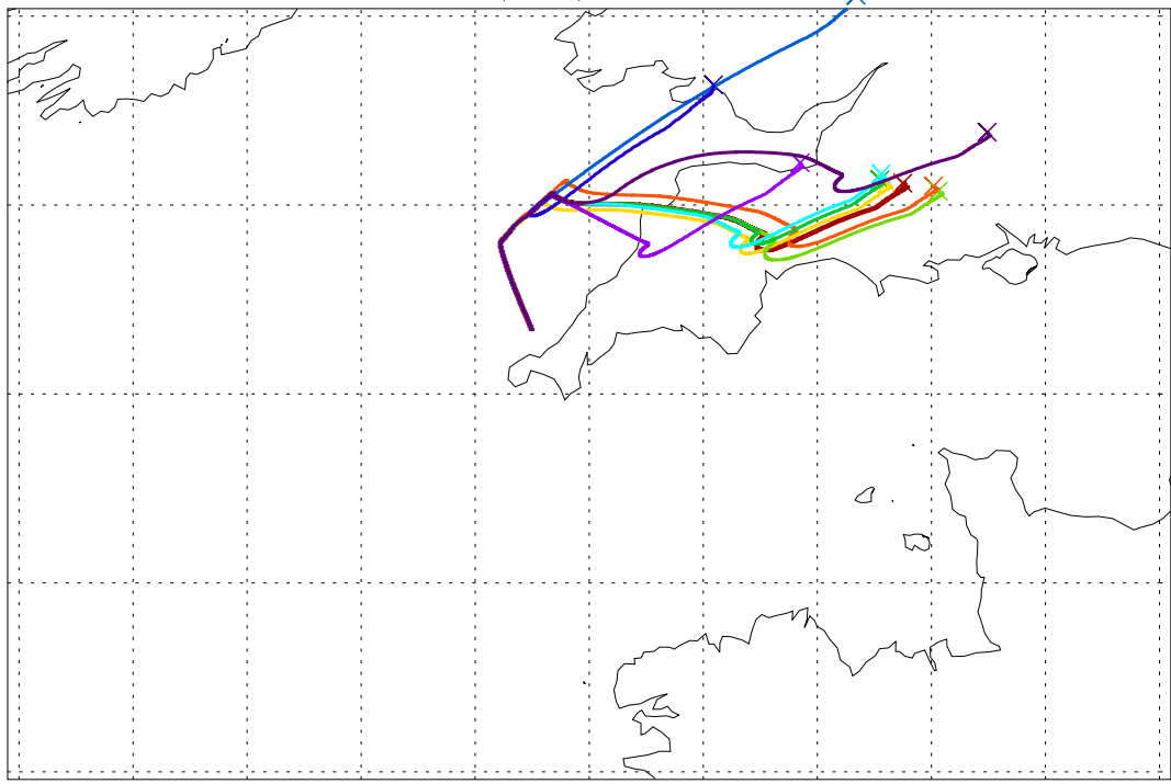
Balloon launch 12UT 14/09/2003 024hr met forecast
