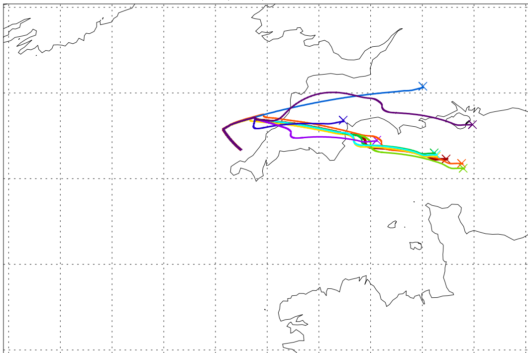
Balloon launch 12UT 15/09/2003 024hr met forecast
