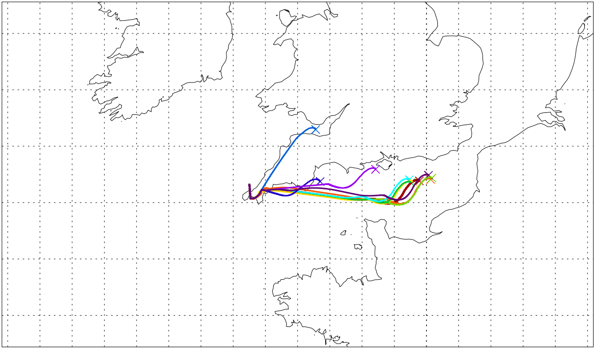
Balloon launch 12UT 27/09/2003 024hr met forecast
