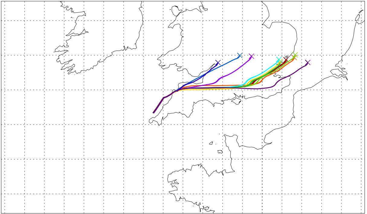
Balloon launch 12UT 29/09/2003 024hr met forecast
