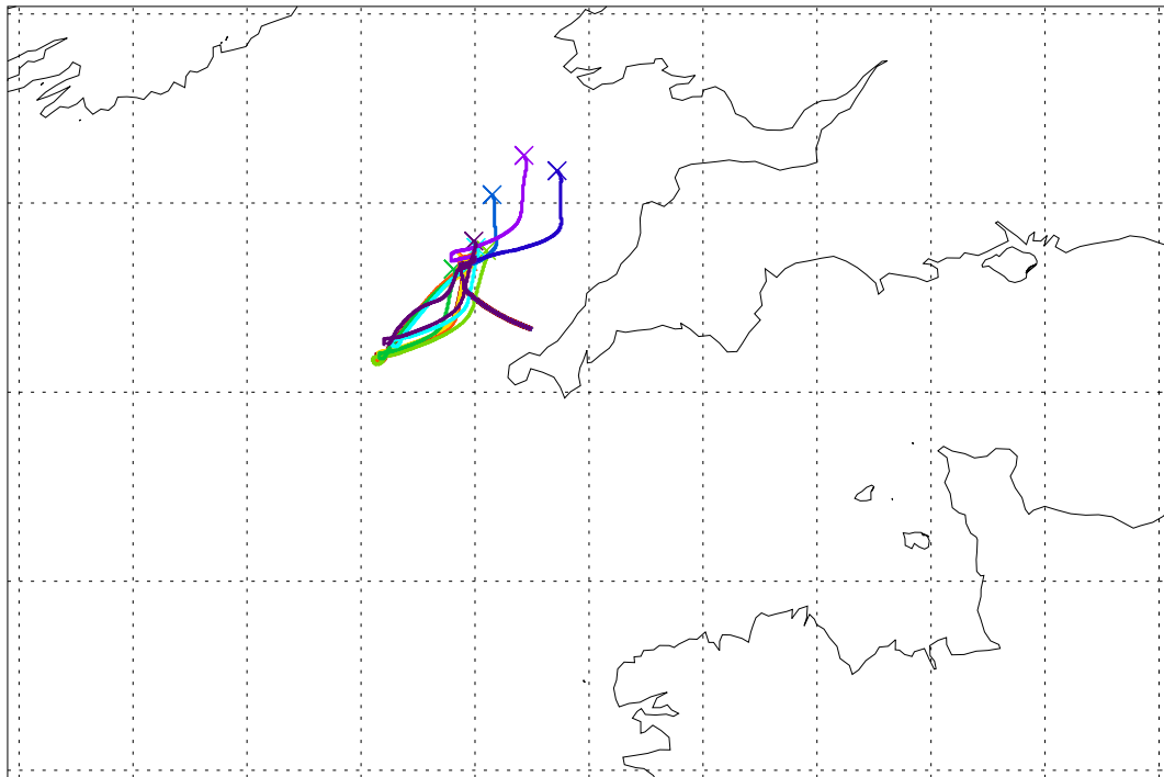
Balloon launch 12UT 04/09/2003 048hr met forecast
