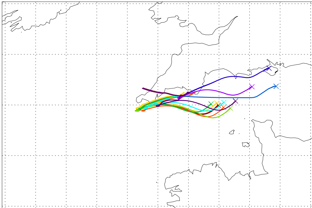
Balloon launch 12UT 06/09/2003 048hr met forecast
