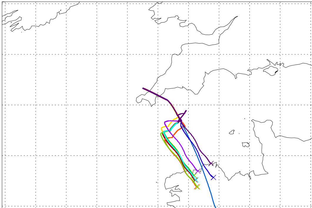
Balloon launch 12UT 10/09/2003 048hr met forecast
