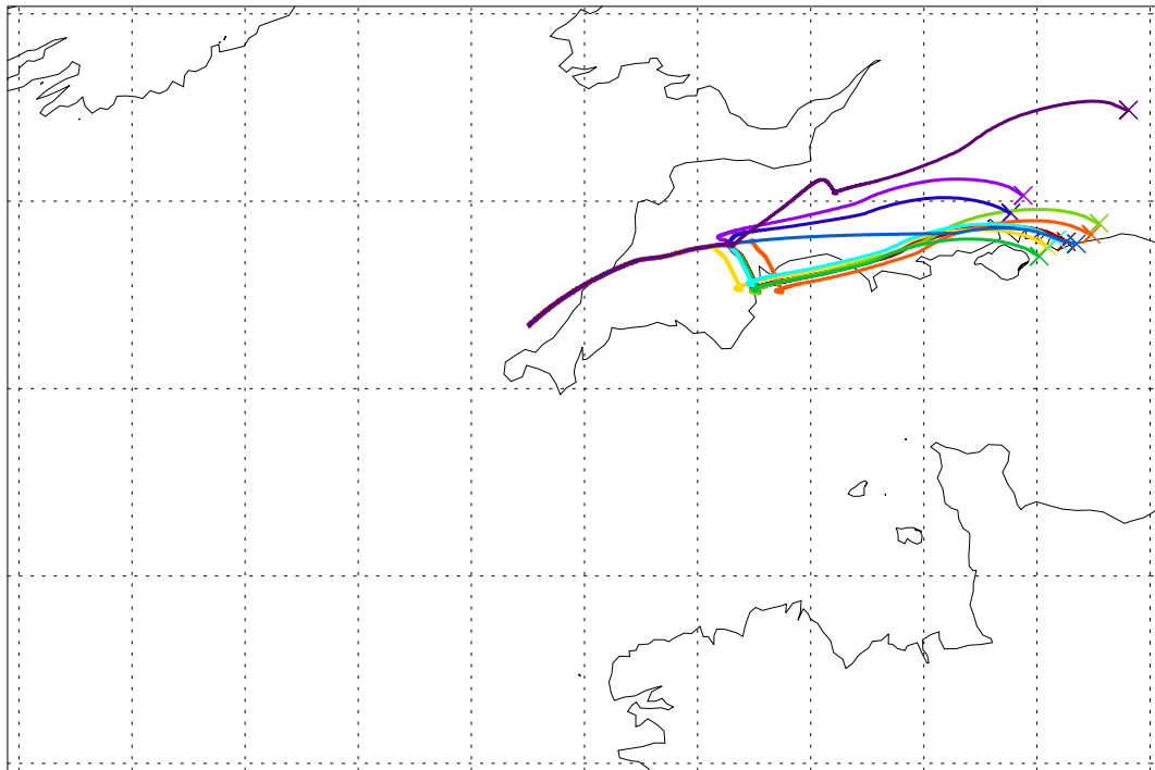
Balloon launch 12UT 11/09/2003 048hr met forecast
