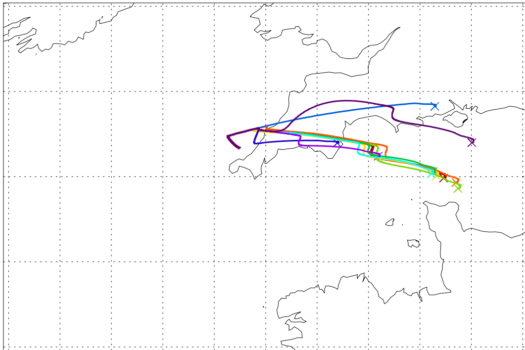
Balloon launch 12UT 15/09/2003 048hr met forecast
