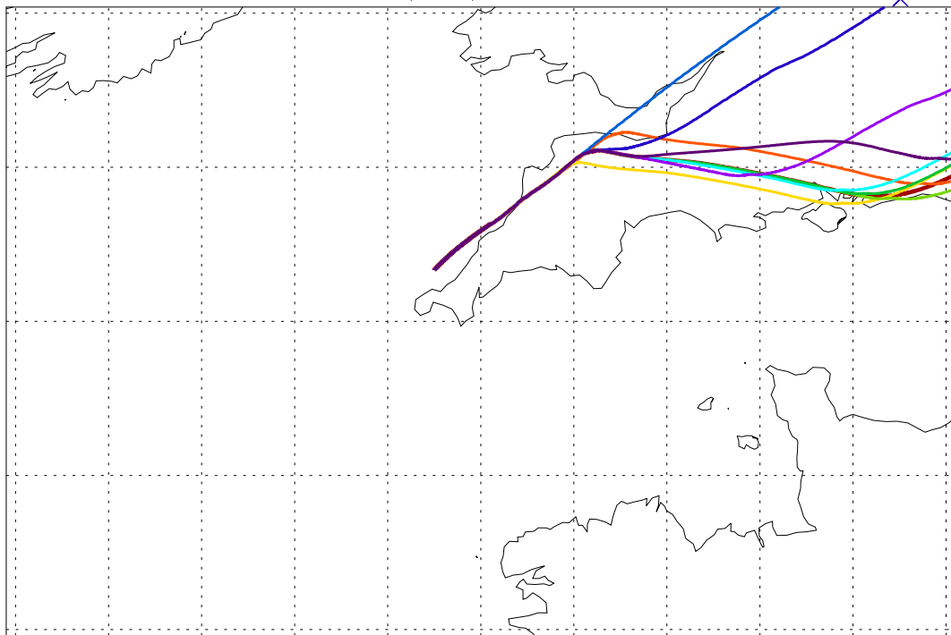
Balloon launch 12UT 18/09/2003 048hr met forecast
