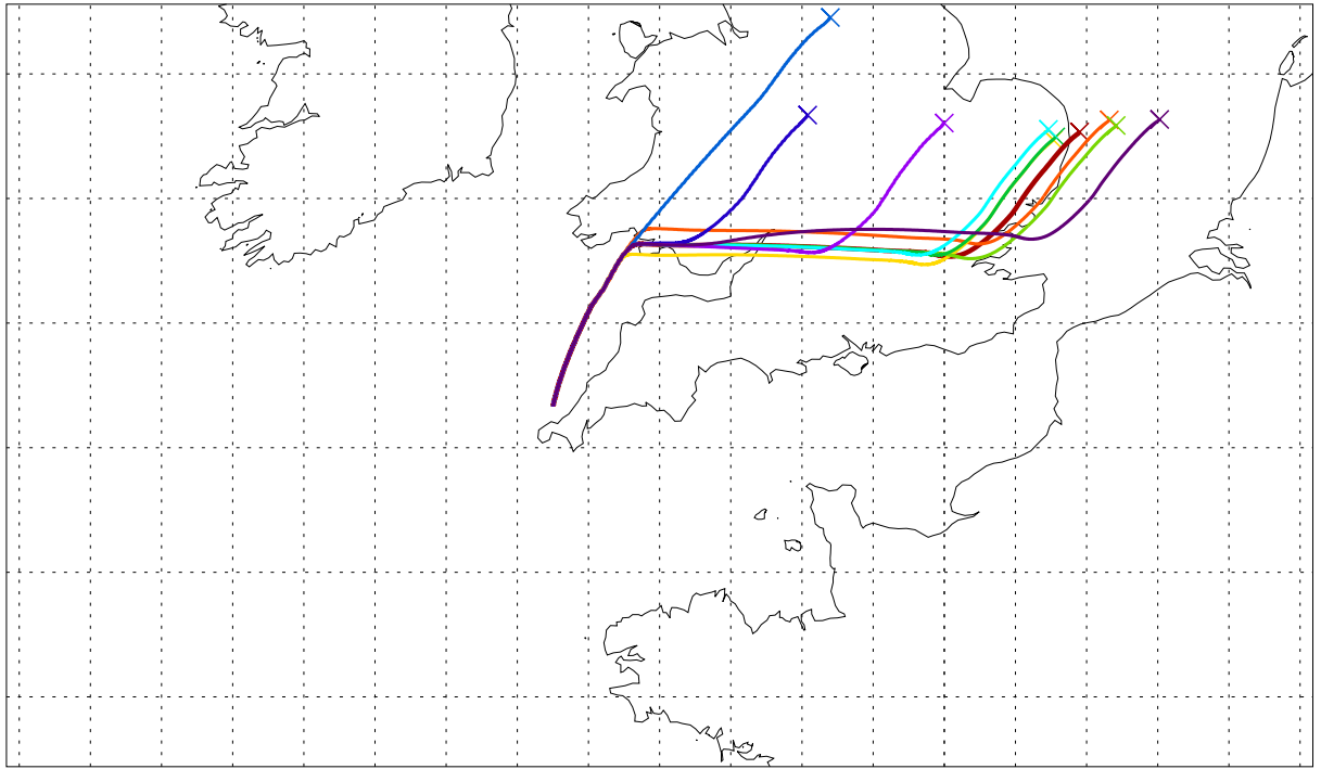
Balloon launch 12UT 21/09/2003 048hr met forecast
