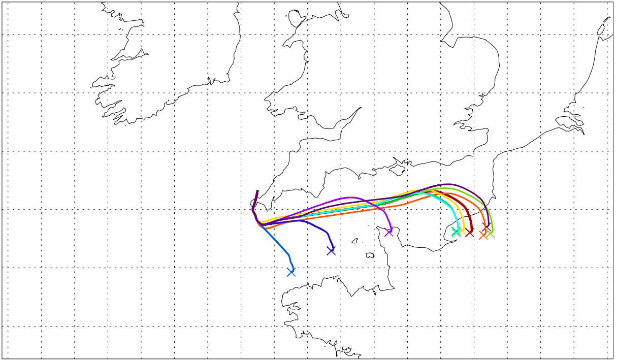
Balloon launch 12UT 23/09/2003 048hr met forecast
