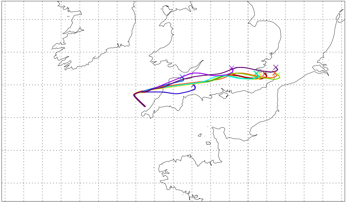
Balloon launch 12UT 24/09/2003 048hr met forecast
