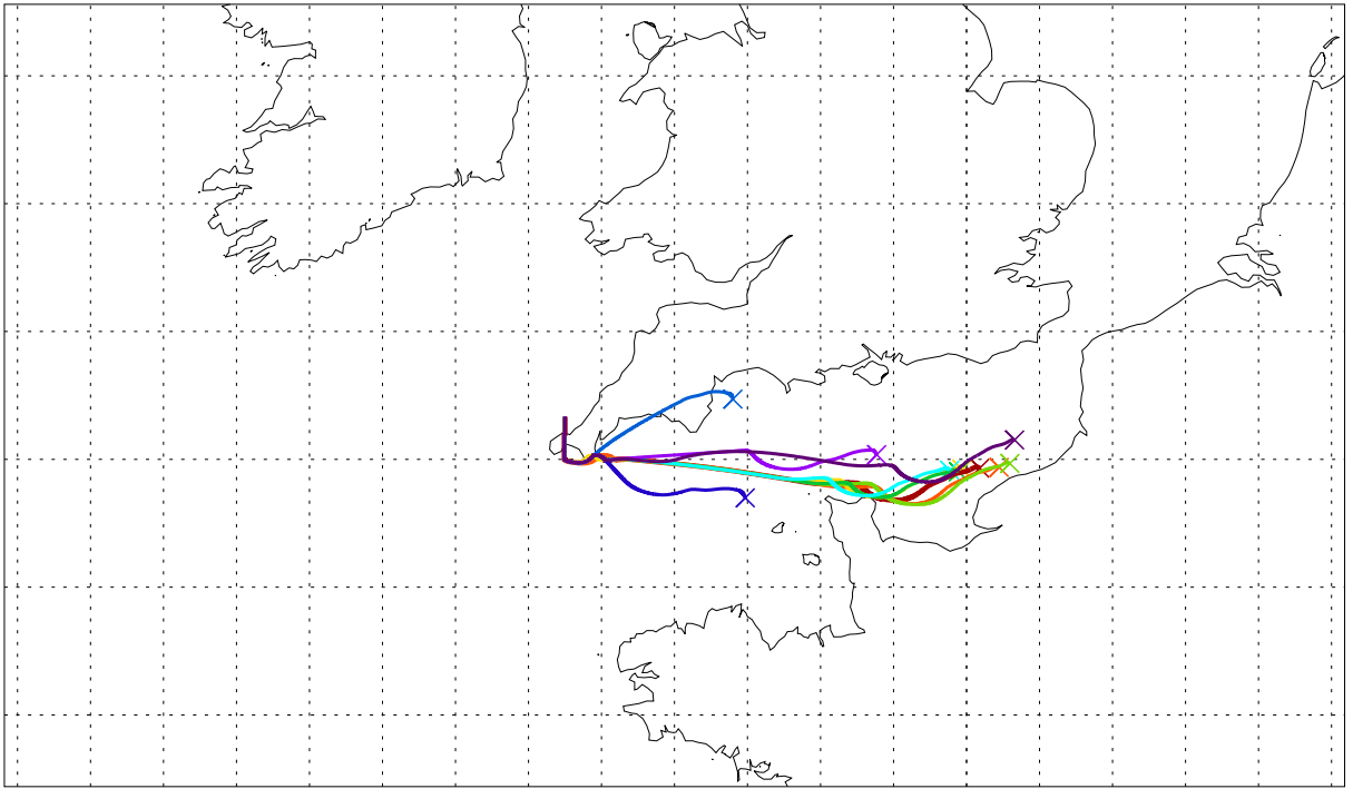
Balloon launch 12UT 27/09/2003 048hr met forecast
