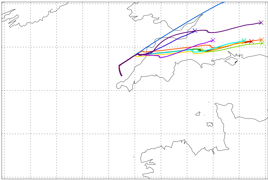
Balloon launch 04UT 15/09/2003 064hr met forecast
