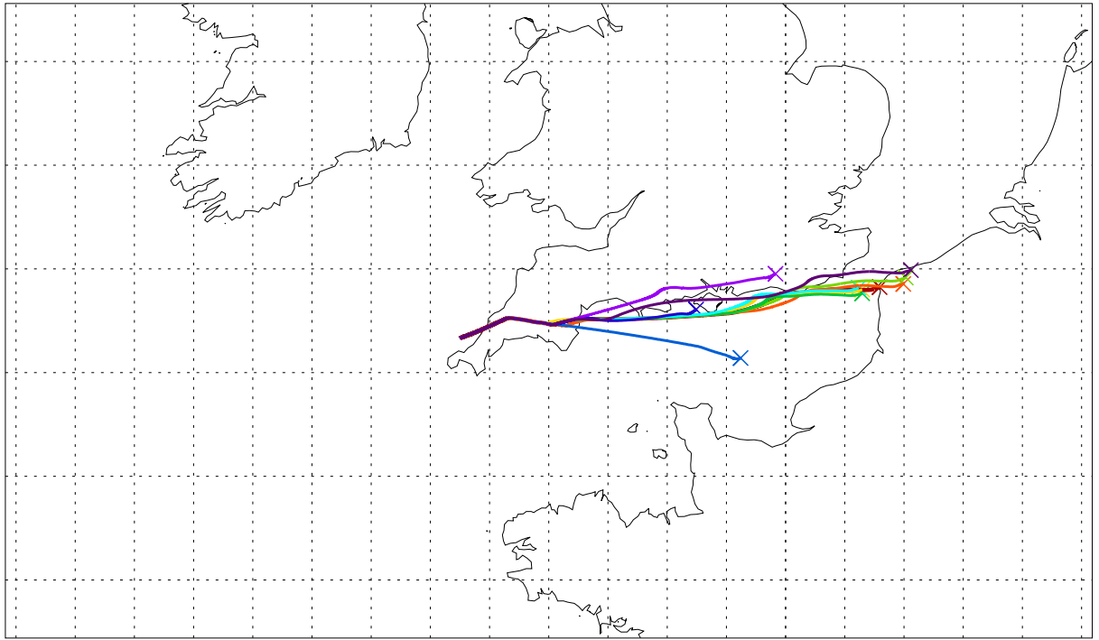
Balloon launch 04UT 29/09/2003 064hr met forecast
