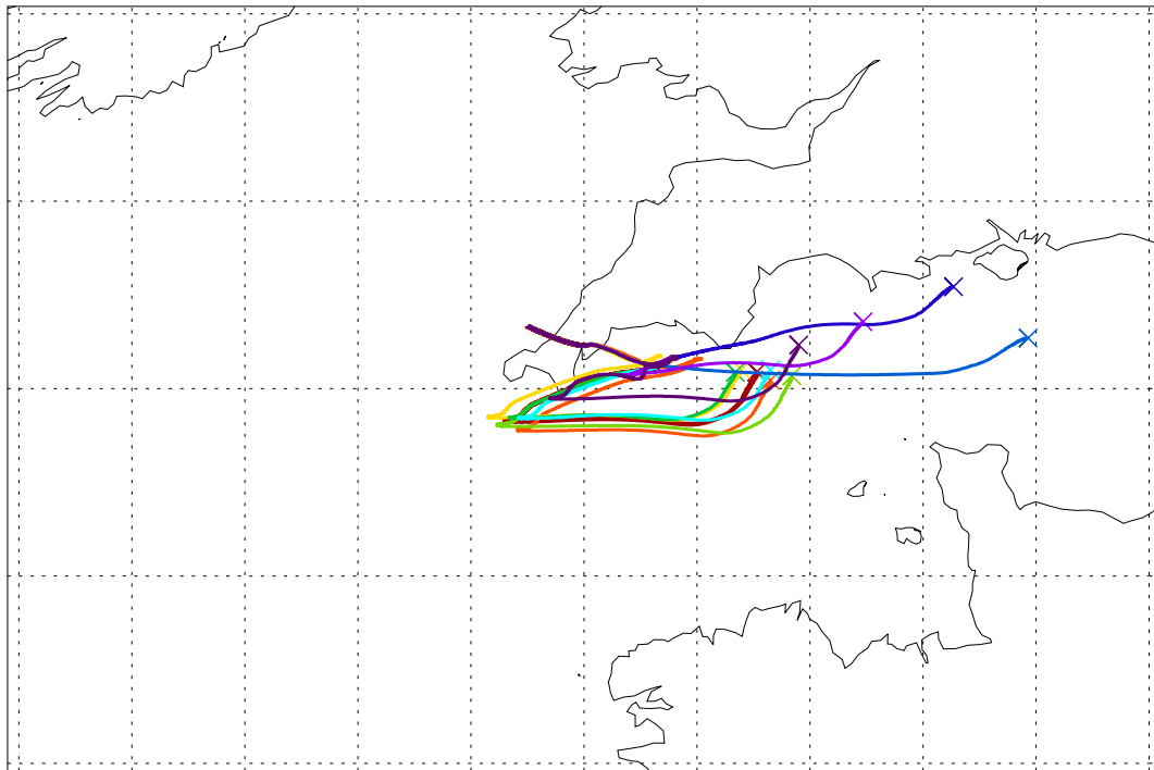
Balloon launch 12UT 06/09/2003 072hr met forecast
