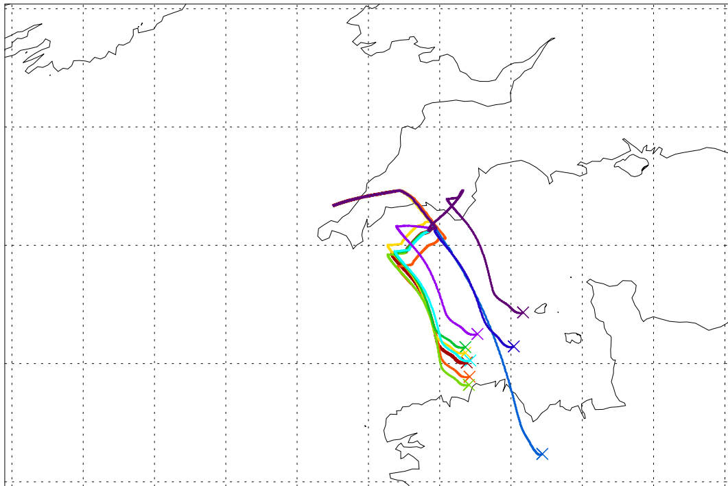
Balloon launch 12UT 10/09/2003 072hr met forecast
