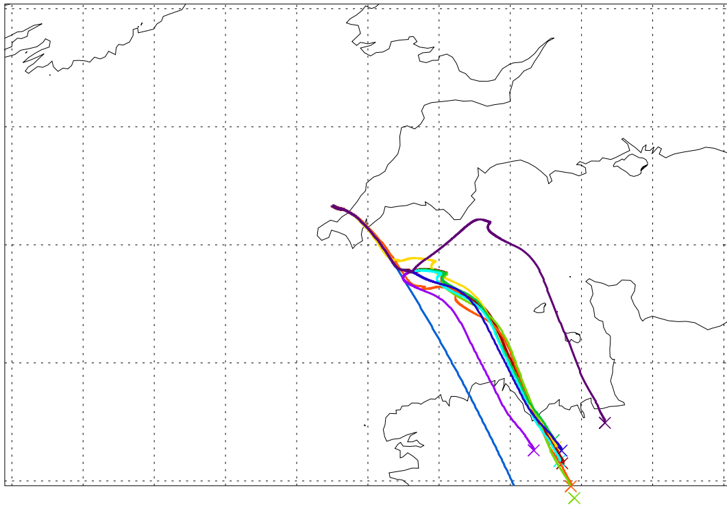
Balloon launch 12UT 12/09/2003 072hr met forecast
