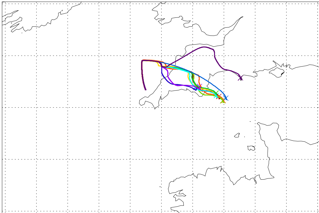
Balloon launch 12UT 13/09/2003 072hr met forecast
