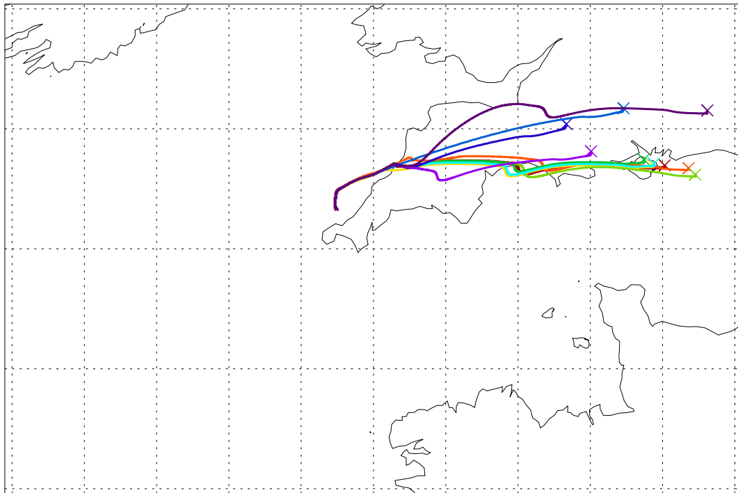
Balloon launch 12UT 14/09/2003 072hr met forecast
