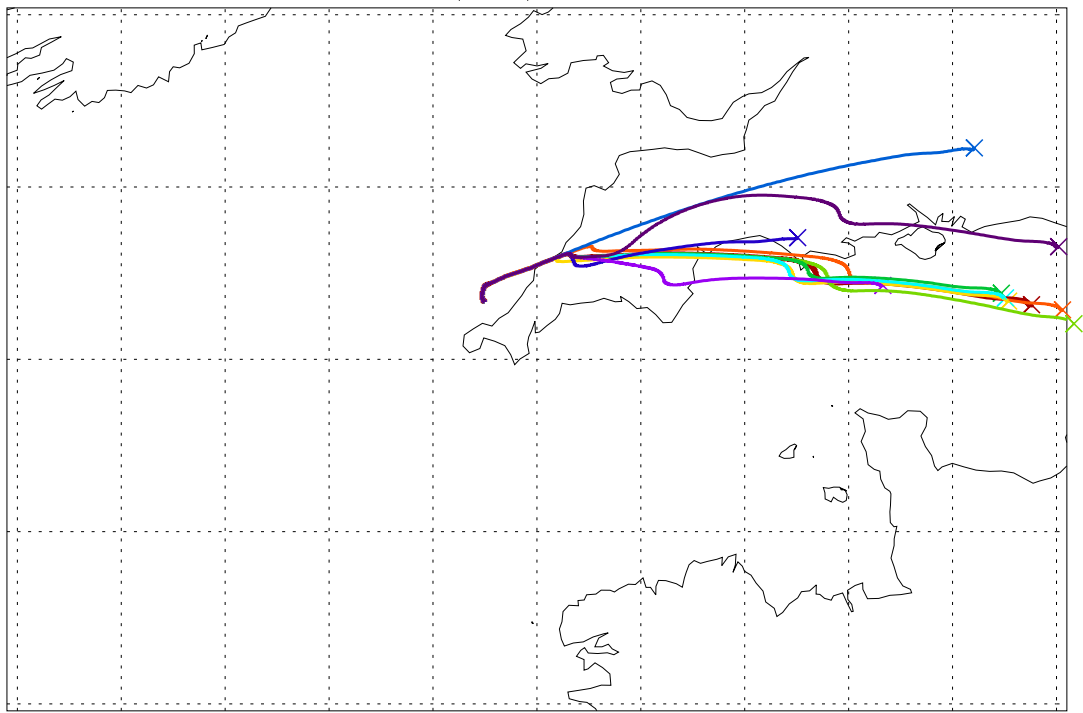
Balloon launch 12UT 15/09/2003 072hr met forecast
