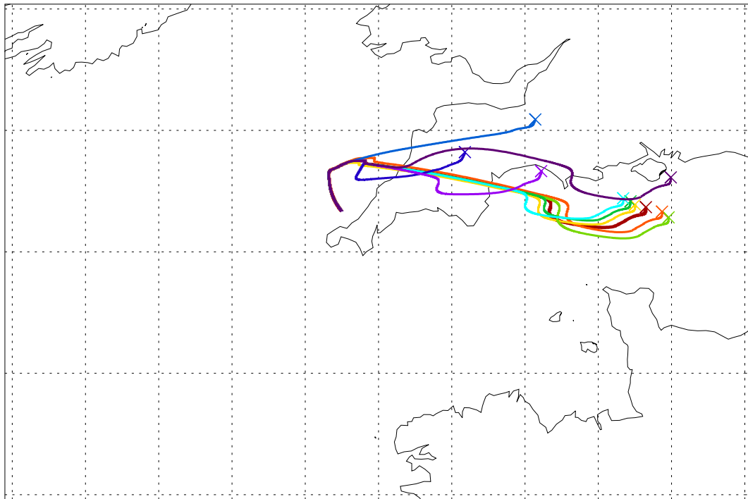
Balloon launch 12UT 16/09/2003 072hr met forecast
