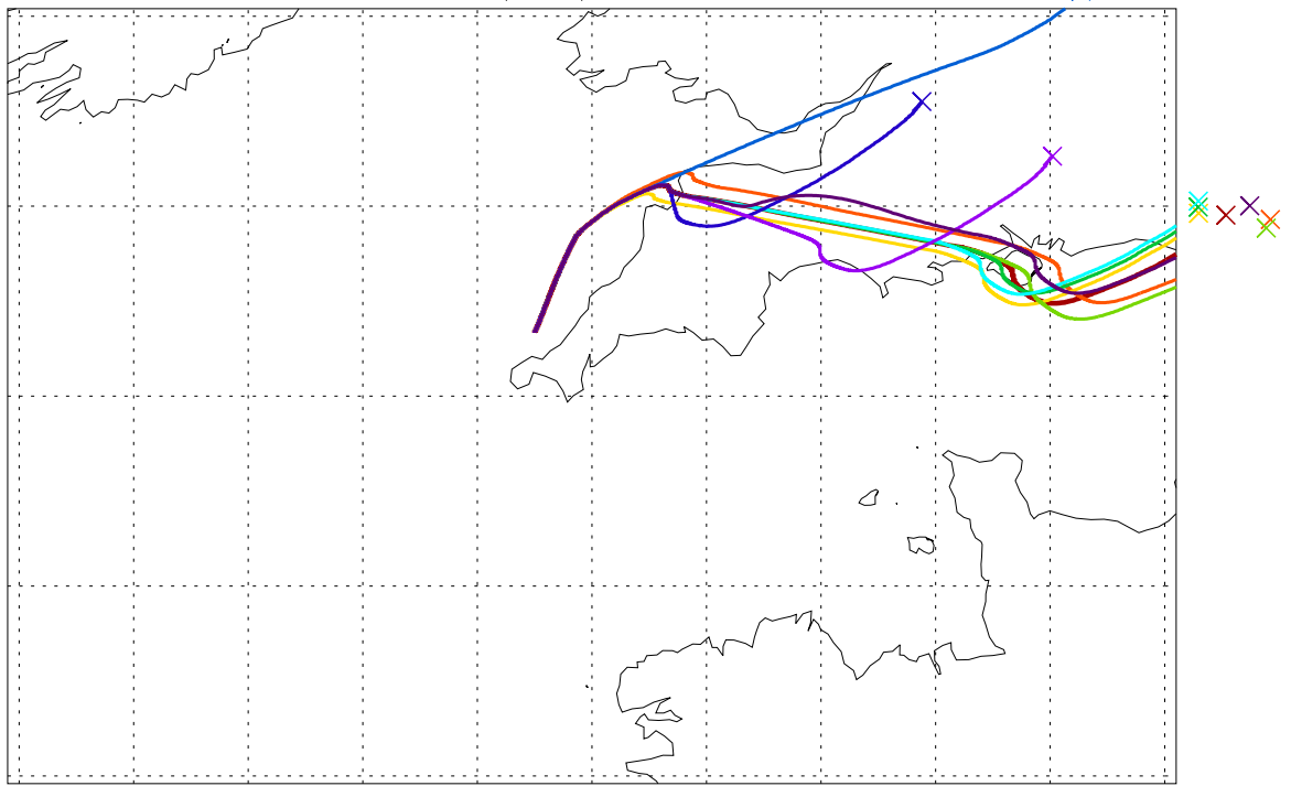
Balloon launch 12UT 17/09/2003 072hr met forecast
