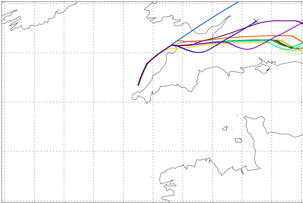
Balloon launch 12UT 19/09/2003 072hr met forecast
