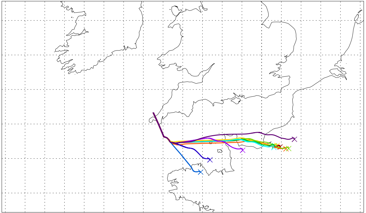
Balloon launch 12UT 22/09/2003 072hr met forecast
