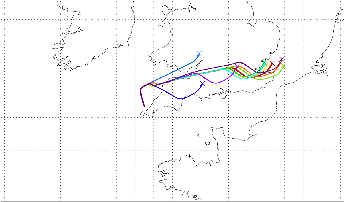
Balloon launch 12UT 25/09/2003 072hr met forecast
