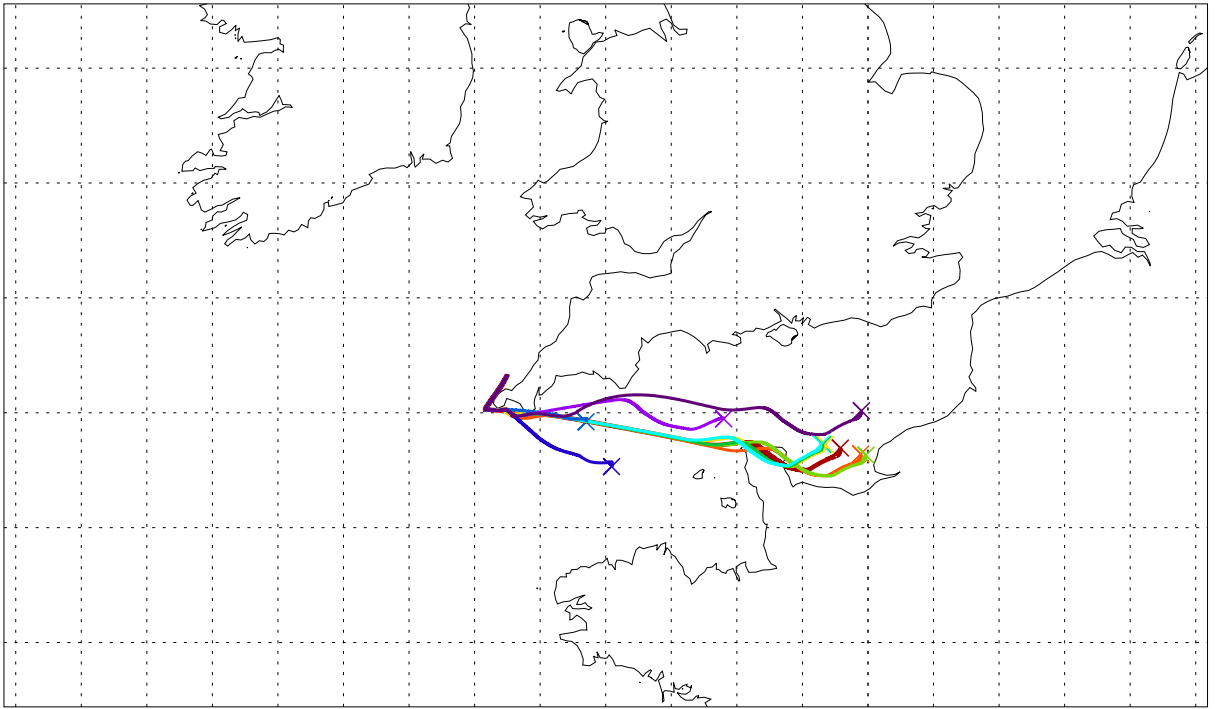
Balloon launch 12UT 27/09/2003 072hr met forecast
