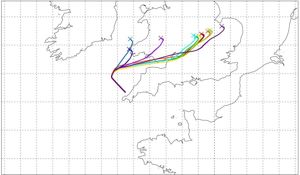
Balloon launch 12UT 30/09/2003 072hr met forecast
