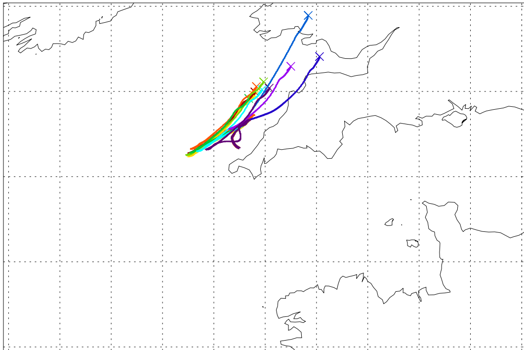
Balloon launch 04UT 05/09/2003 088hr met forecast
