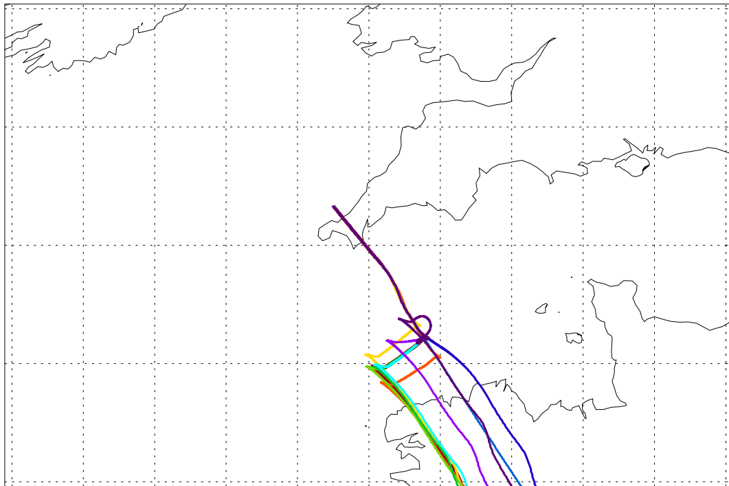
Balloon launch 04UT 09/09/2003 088hr met forecast
