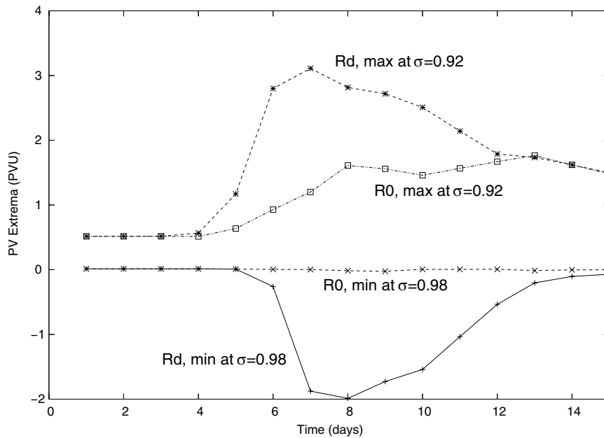
Figure 7. Time series of extreme values of potential vorticity during the life cycles R0 and Rd. Maximum values are shown for the surface \sigma = 0.92 and minimum values for the surface \sigma = 0.98 .
