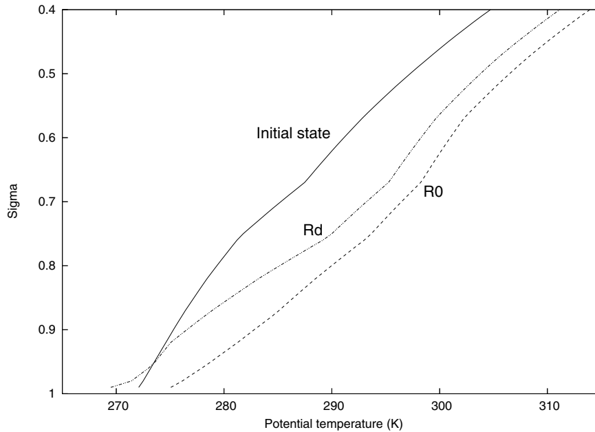
Figure 12. Profiles of the zonal-mean potential temperature averaged between latitudes 50^\circ and 70^\circ\text{N} , for the initial state (solid) and for runs R0 (dashed) and Rd (dotted), averaged between 15 and 20 days.
