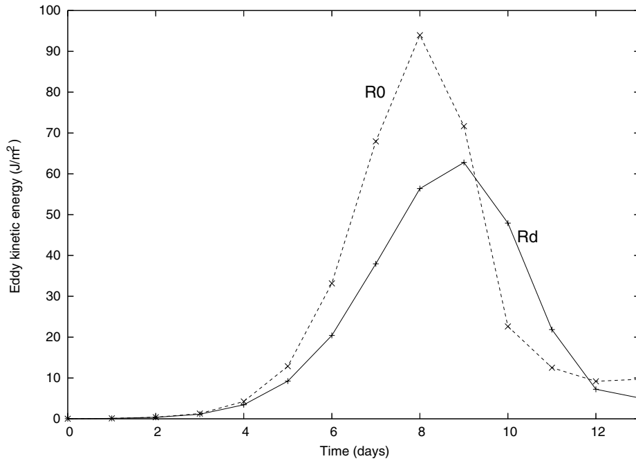
Figure 3. The domain-averaged eddy kinetic energy during life cycles R0 and Rd.
