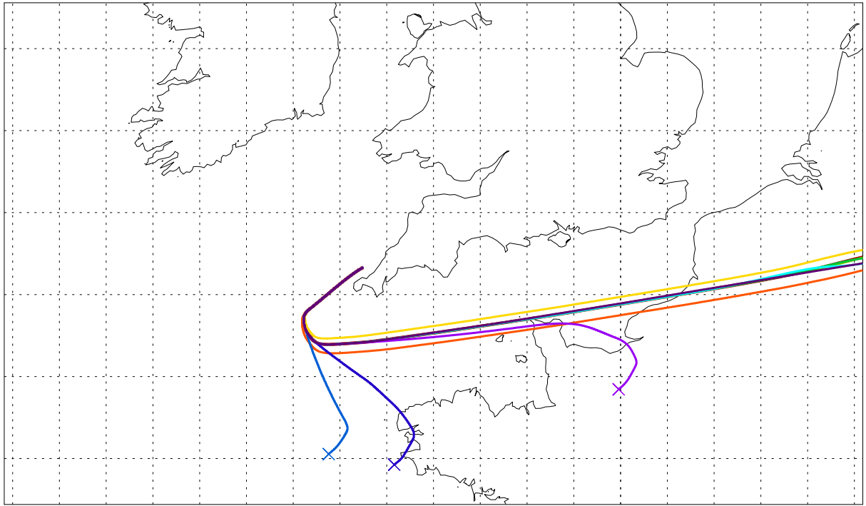
Balloon launch 12UT 23/10/2003 048hr met forecast
